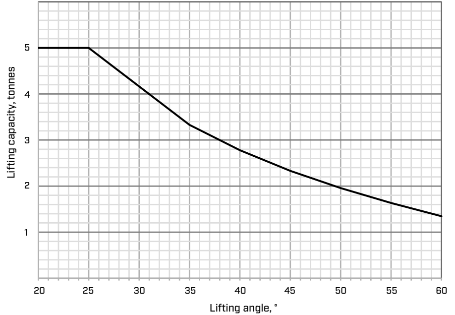
Max load Aluex STR5 WLL 5t
