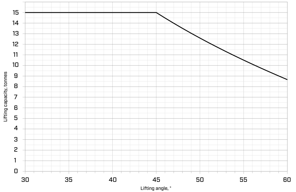
Max Load Aluex STR15 WLL 15t
